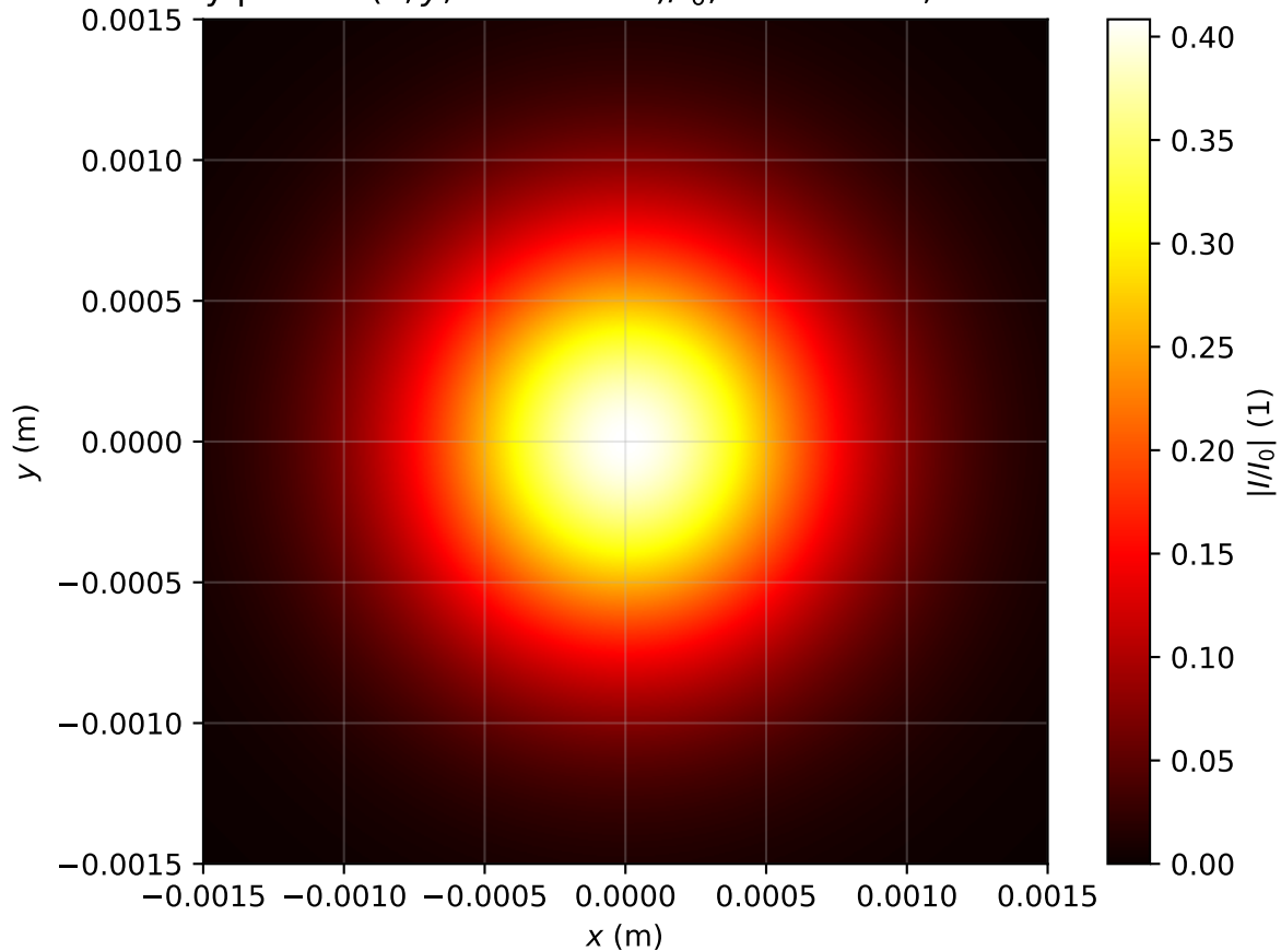
Intensity profile I(x, y, z = 3.423m)/I_0 , P_{in}=0.4P_{cr} , artificial time
